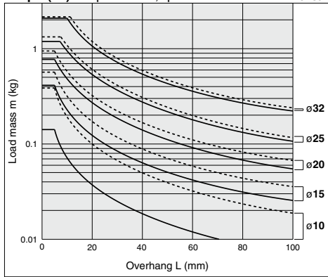
Graph (14) V = Over 400 mm/s; Up to 75 mm stroke ——— CXSJM ----- CXSJJL
