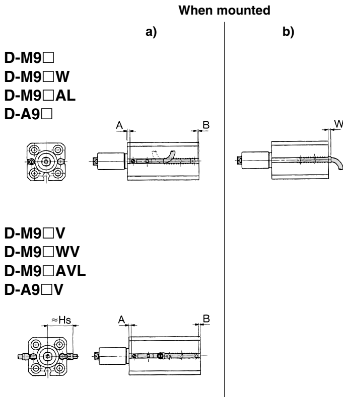
Auto Switch Proper Mounting Position
