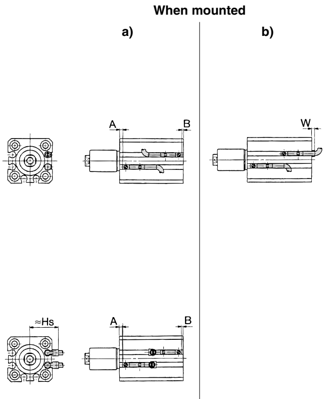
Auto Switch Mounting Height
